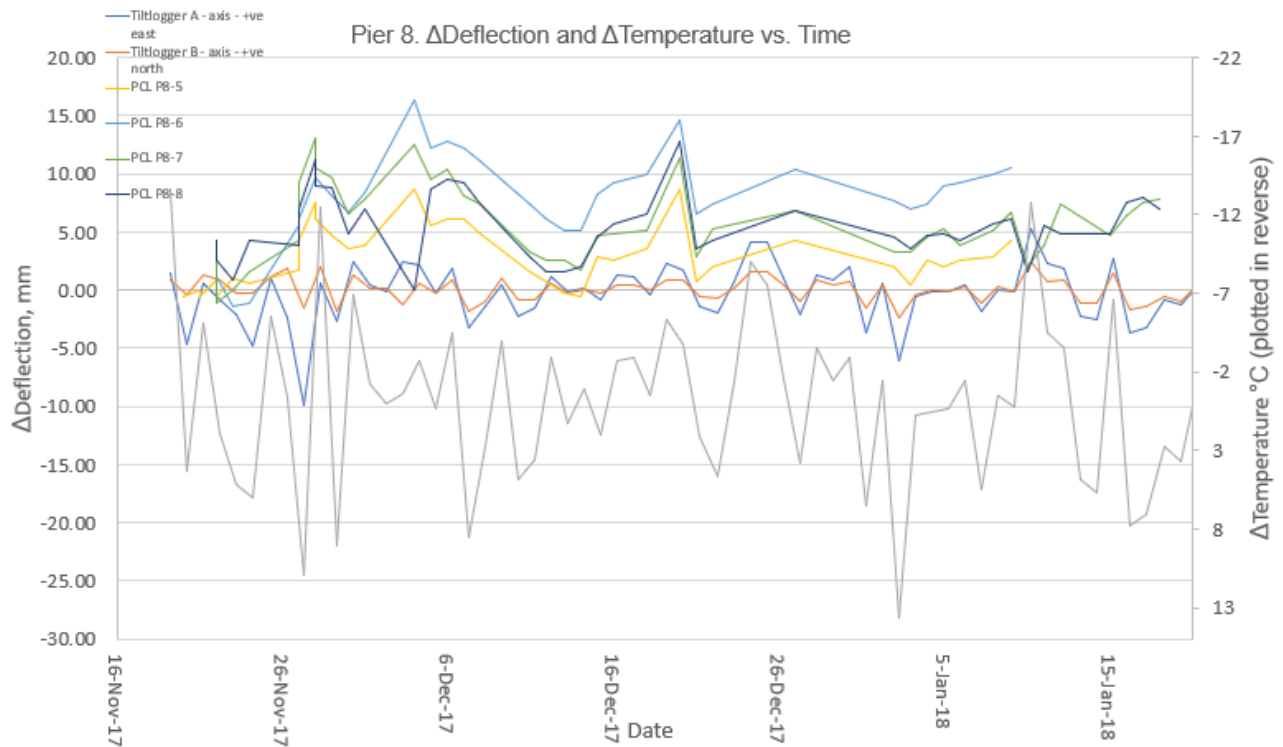
Figure 5 – Tilt, Survey and Temperature Data, Pier 8
