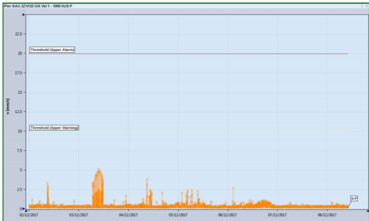
Figure 4 – Typical Vibration Monitoring Data
