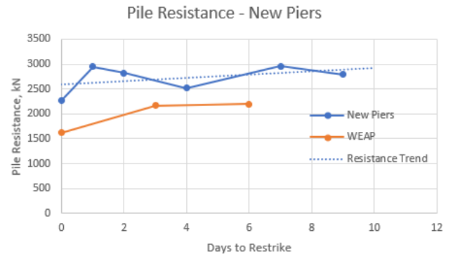
Figure 3 – Pile Resistance, New Piers
