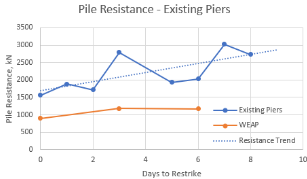
Figure 2 – Pile Resistance, Existing Piers
