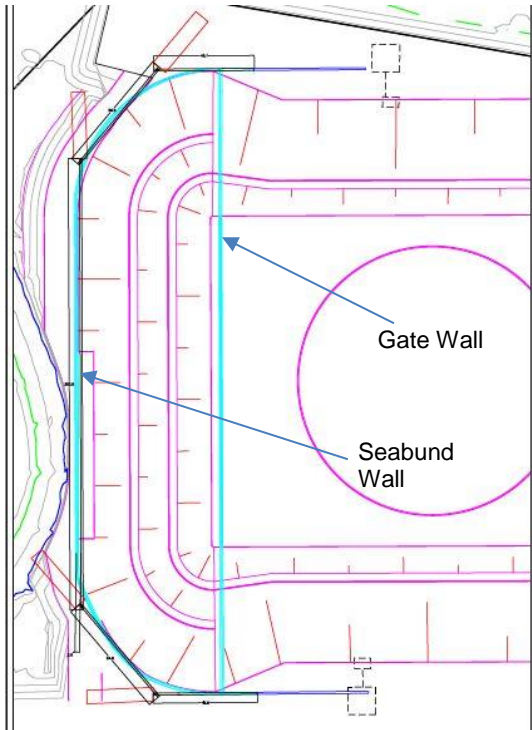
Figure 2. The final cutoff wall alignments shown in blue and teal
