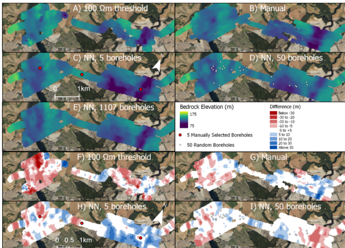
Figure 2: Bedrock elevation models produced from five different methods, focusing on the river crossing at Vormaa and Uää as well as differences between the most accurate model (NN using 1107 boreholes) and the other four models. Negative values indicate that the final model is lower, and vice versa.
