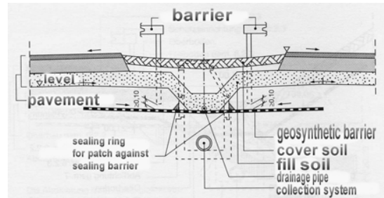
Figure 2. Basic drawing for a road cross-section zone III "central reserve"
