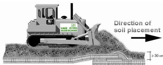
Figure 3. Schematic soil placement over a GCL
