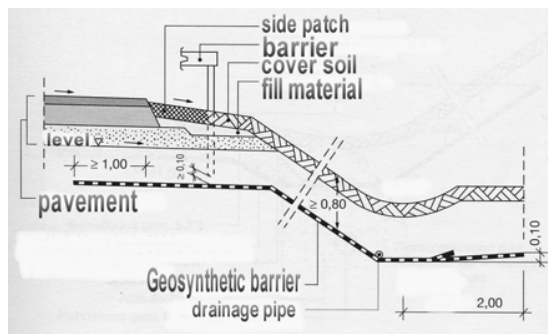
Figure 1. Basic drawing for a road cross-section zone III "drainage over the slope"
