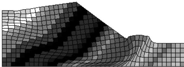
Figure 9. Parallel failure mechanism #1
