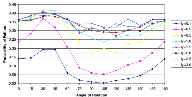
Figure 4. Probability of failure vs. angle of rotation
