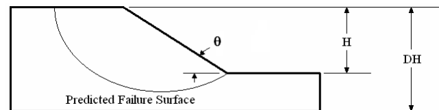
Figure 6. Predicted failure surface
