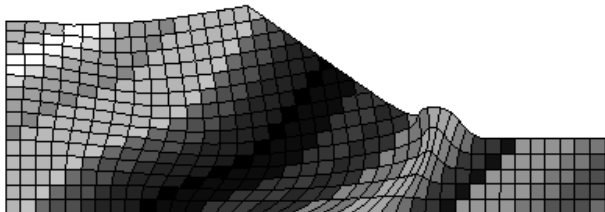
Figure 10. Parallel failure mechanism #2
