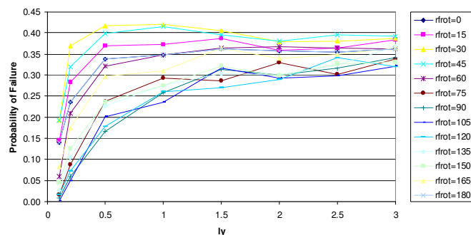
Figure 5. Probability of failure vs. spatial correlation
