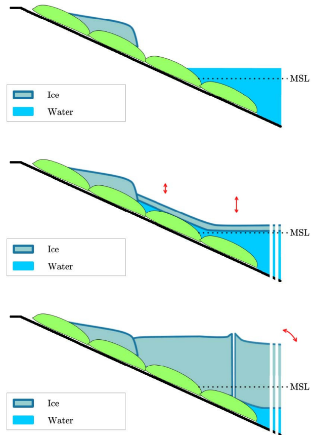
Figure 14. Profile of the bags during the ice cover period at resp. freeze-up, low tide and high tide from top to bottom (Caline, 2010)
