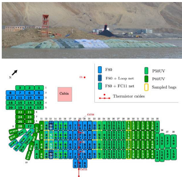
Figure 7. View and map of breakwater after construction (September 2006).
