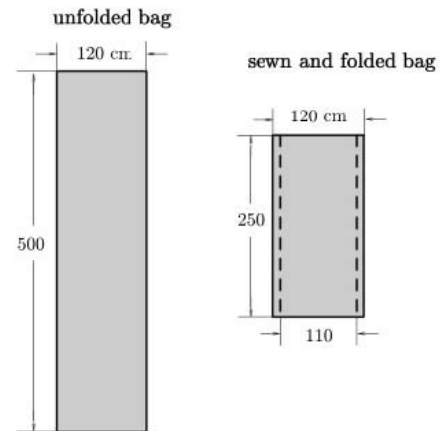
Figure 5. Sketch of the geobags used at Barryneset.
