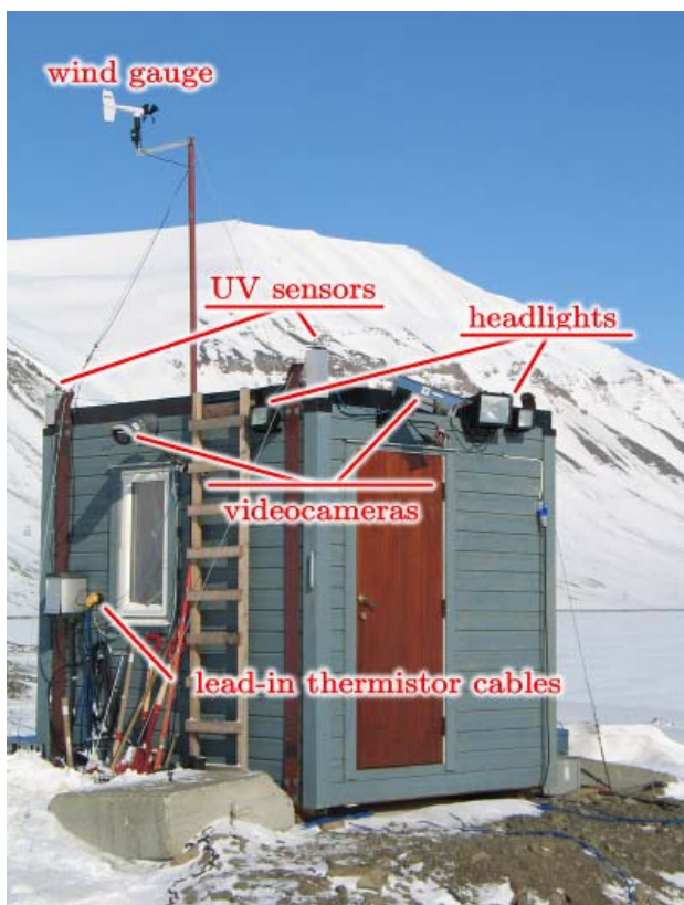
Figure 8. Weather station and instrumentation hut (September 2006).
