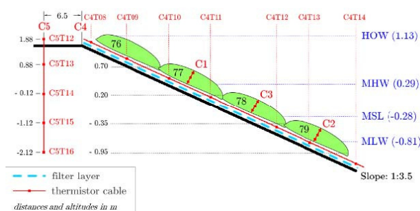
Figure 10. Profile of the breakwater slope covered with bags
