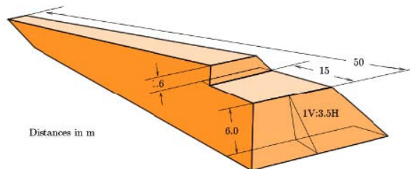
Figure 4. Sketch of the breakwater (Caline, 2010).
