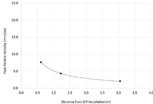
Figure 2. Ground Vibration Monitoring Adjacent to Installations
