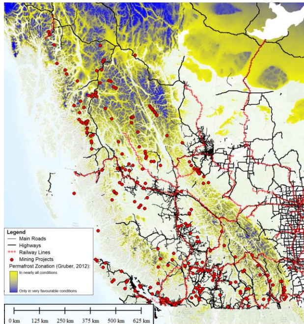
Figure 3. Transportation infrastructure, mining projects and permafrost in western Canada. Permafrost zonation from Gruber (2012).
