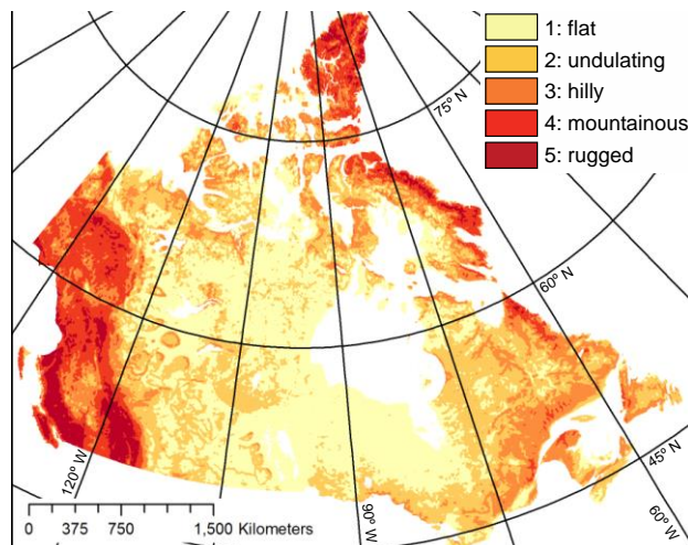
Figure 1. Terrain ruggedness map of Canada (Gruber 2012). Equivalents to the classes shown are: Rugged (5): e.g., Mt. Robson in Banff National Park; Mountainous (4): Pelly mountains, NE of Whitehorse; Hilly (3): Iqaluit; Undulating (2): Yellowknife; Flat (1): Mackenzie delta.
