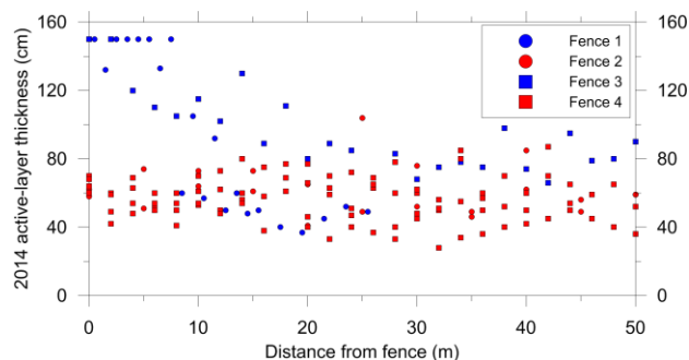
Figure 5. Active-layer thicknesses along transects at all fences in 2014. The blue data points are from sites on flat ground and the red points are from sites on slopes.
