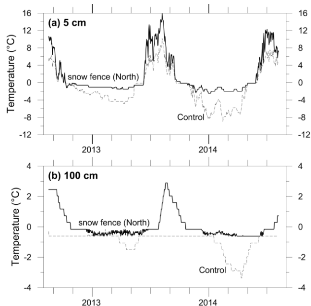
Figure 4. Ground temperatures at (a) 5 cm and (b) 100 cm depth near the snow fence and at the control site.
