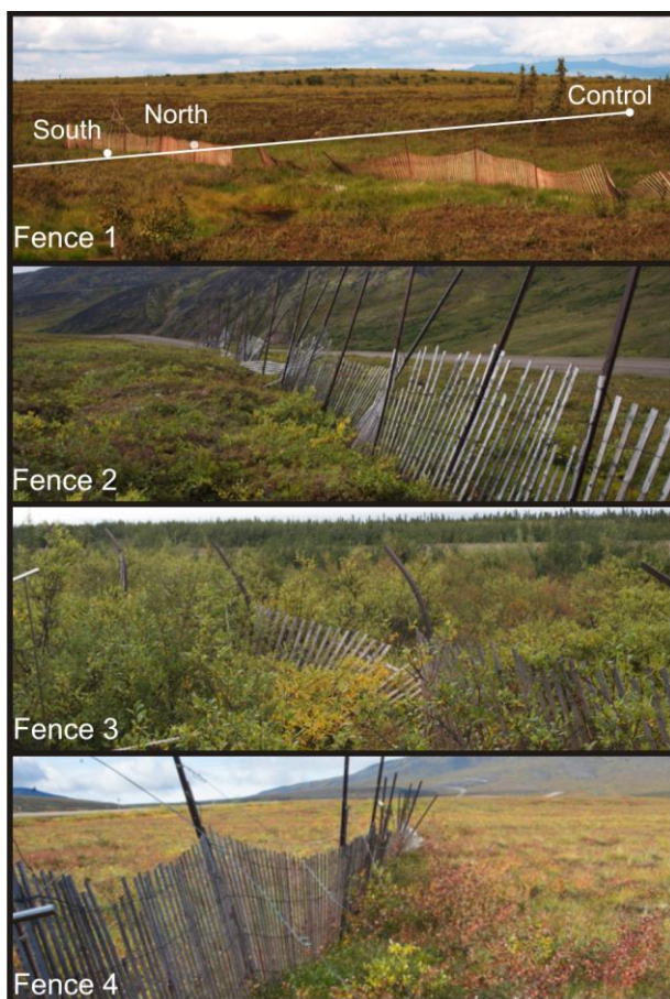
Figure 2. Field sites in summer 2014. Locations of the transect (line) and shallow thermistor arrays (dots) are shown for Fence 1.
