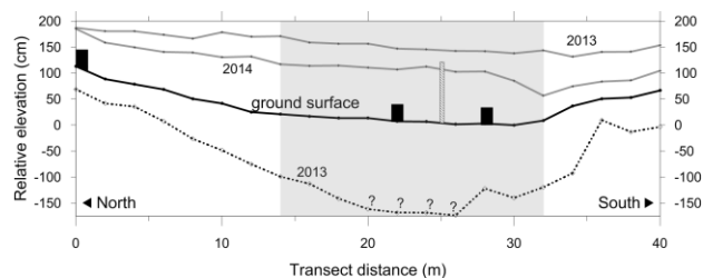
Figure 3. Cross-section of Fence 1 showing the ground surface, snow depths, and active-layer thicknesses along the transect. The gray shading represents sedge-dominated vegetation. Thermistor arrays are shown as black rectangles.
