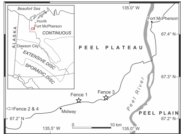
Figure 1. Location of study sites. Fences 2 and 4 are at approximately 67.179^{\circ}\text{N} 135.776^{\circ}\text{W} and 67.104^{\circ}\text{N} 136.096^{\circ}\text{W} , respectively, in Richardson Mountains.
