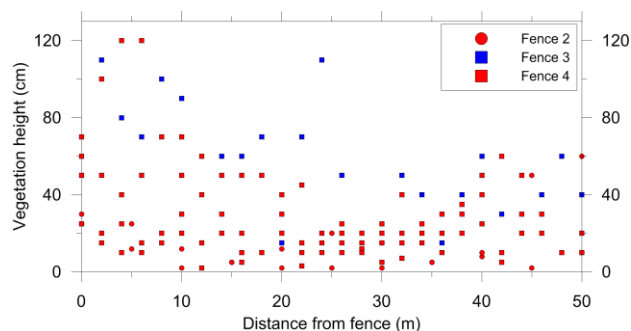
Figure 6. Vegetation heights along transects at Fences 2-4. The blue data is from the site in flat ground and the red data are from sites on slopes.
