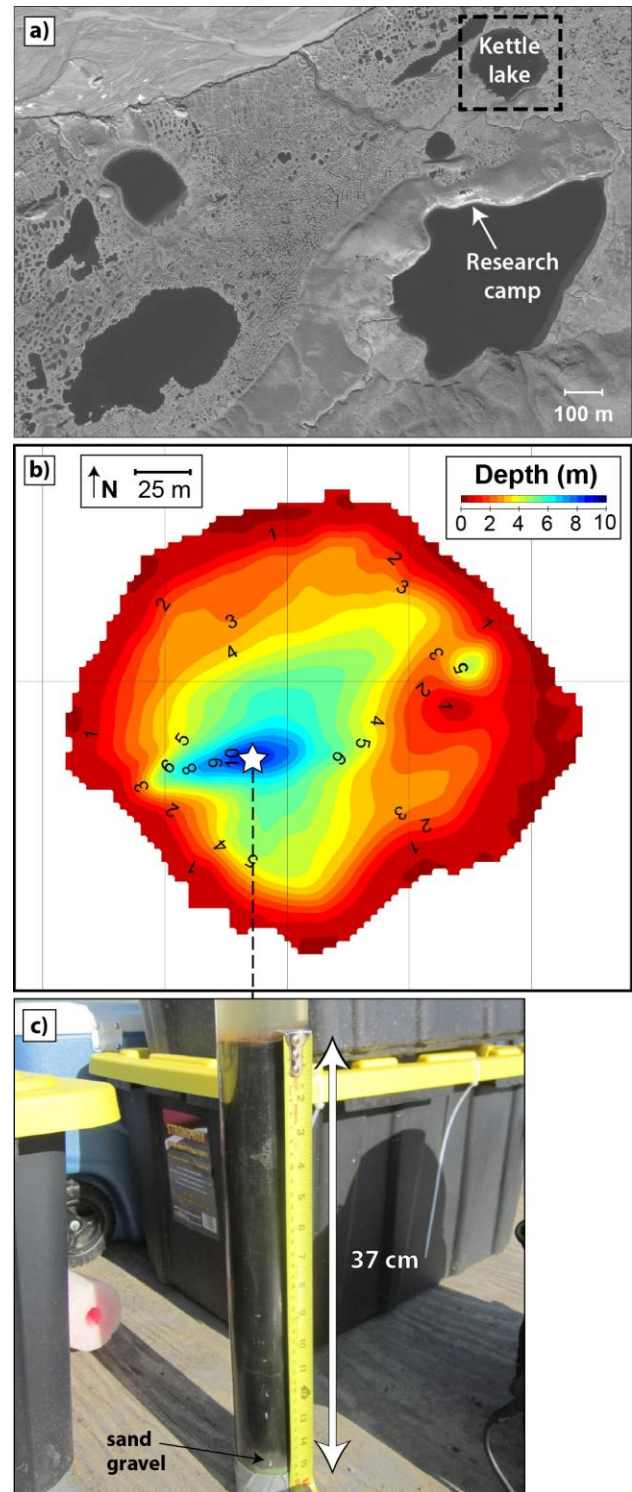
Figure 5. Paleolimnological sampling in a kettle lake of the Canadian Arctic. (a) Satellite image (GeoEye-1, 18 July 2010) showing the sampled kettle lake within a glacial valley (Bylot Island, Nunavut; Figure 1). (b) Bathymetric map generated using the above-mentioned GPS-sonar system. (c) Photo of a 37-cm long sediment core collected from the deepest part of the lake (white star on the map).
