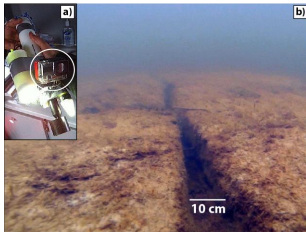
Figure 4. Lake bottom imagery using a waterproof HD camera. (a) Installation of the camera (circled) on a RBR conductivity-temperature-depth profiler, with lights fixed on the sides. (b) Photograph of the bottom of a thermokarst lake (Bylot Island, Nunavut; Figure 1), showing submerged ice-wedge polygons (~ 1 m depth) and degraded frost crack troughs.
